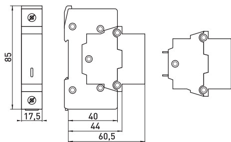
e.industrial.surge.spb
