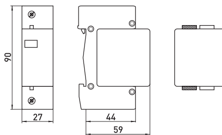
e.industrial.surge.spi.100.npe
